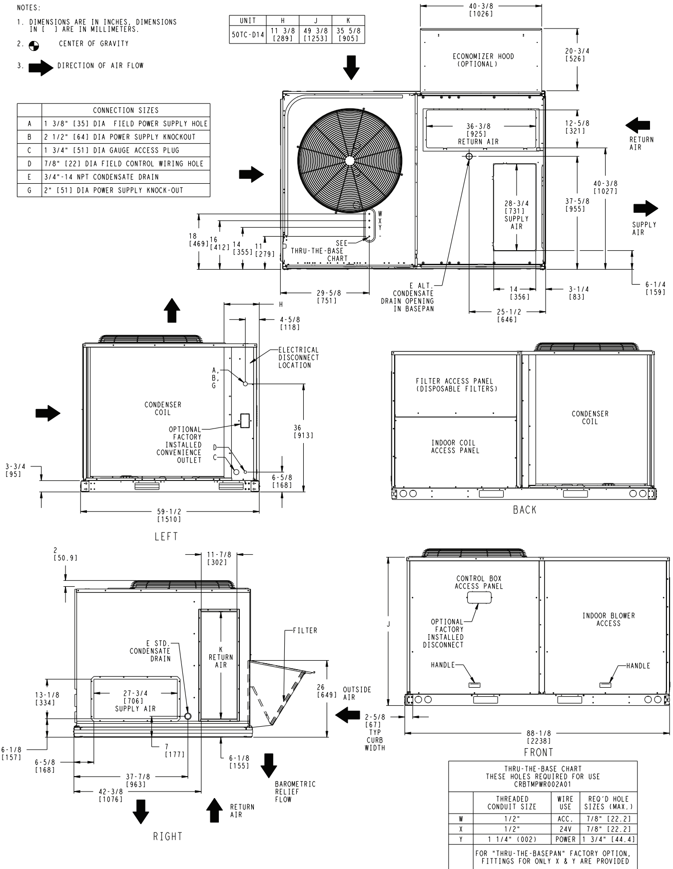
Fig. 11 - Dimensions 50TC 14
