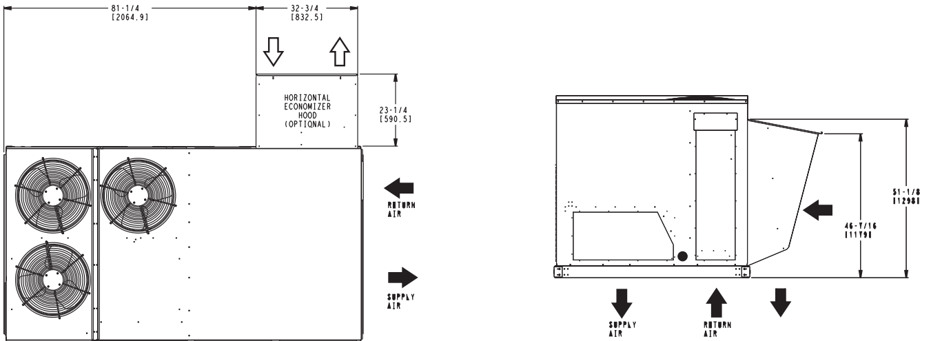
Fig. 15 - Dimensions 50TC 16
